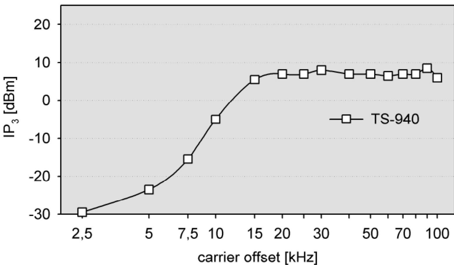
Third order intercept point ( IP_3 ) of Kenwood TS-940, QRG 14.100 MHz, carrier offset 2,5-100 kHz
